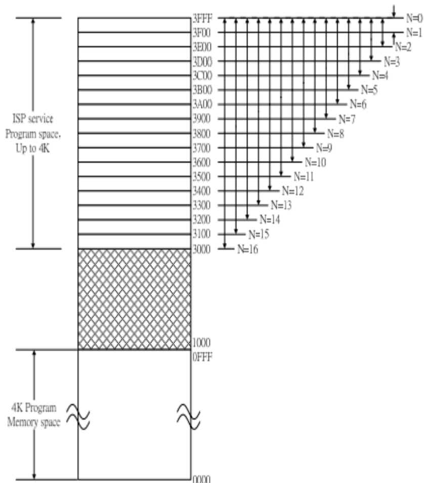
Fig.3.1: Flash Memory Structure
