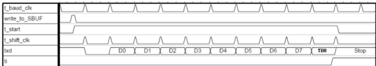
Fig. 9-7: Transmit mode A for Serial 1
