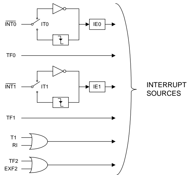
FIGURE 19: INTERRUPT SOURCES
