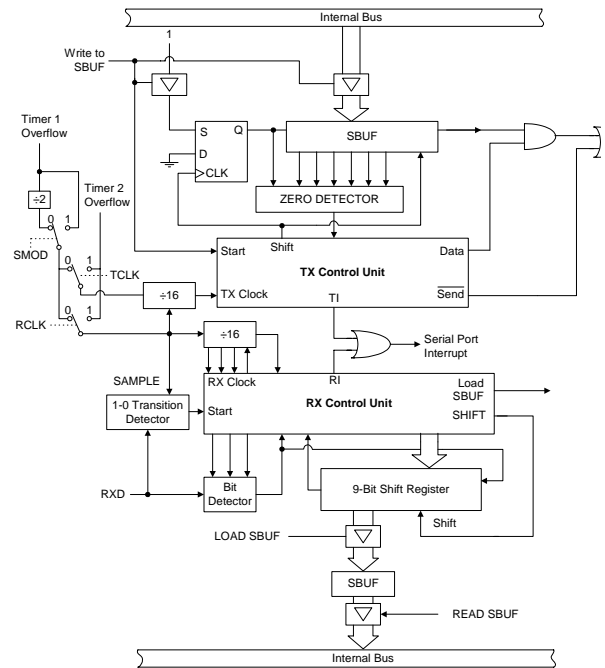
FIGURE 18: SERIAL PORT MODE 3 BLOCK DIAGRAM
