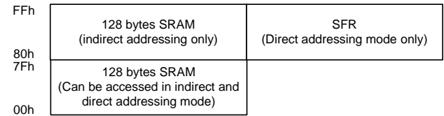
FIGURE 2: CRD89x51 DATA MEMORY
