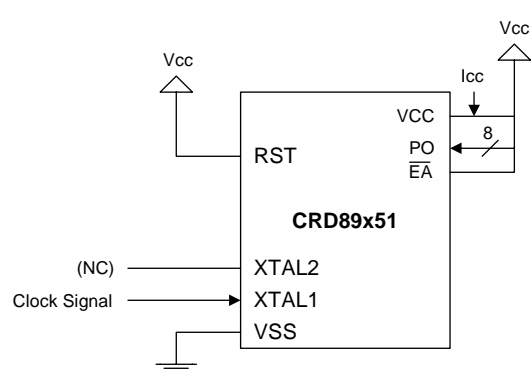
FIGURE 21: ICC ACTIVE MODE TEST CIRCUIT
