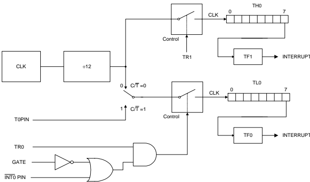
FIGURE 11: TIMER/COUNTER 0 MODE 3
