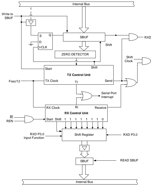
FIGURE 15: SERIAL PORT MODE 0 BLOCK DIAGRAM
